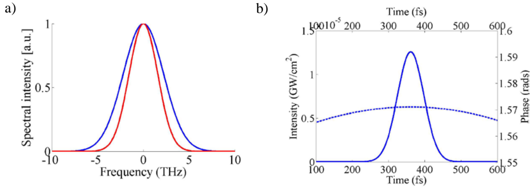
Fig 4. 7: a) Comparison between the spectral intensity of the fundamental (red) and the SH (blue) and b) time characteristics of the SH when using a 10 \text{ }\mu\text{m} thick BBO and 0.5 \text{ GW/cm}^2 peak intensity pulses. In panel b) the dotted line represents the phase and the solid line the intensity.
