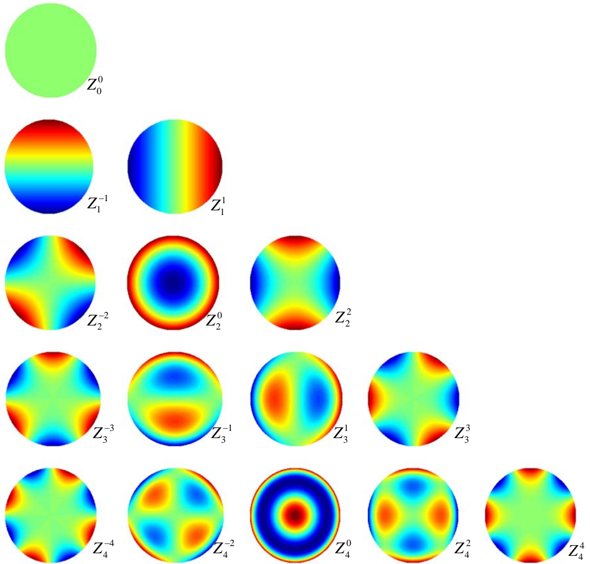
Fig C. 1: Zernike polynomials
