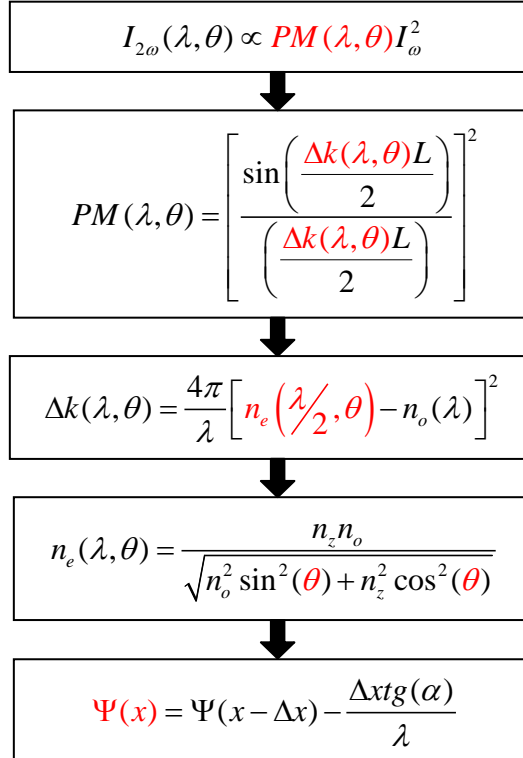
Fig 5. 5: Summary of the retrieval algorithm to compute the wavefront. The quantities calculated in each step are marked in red.
