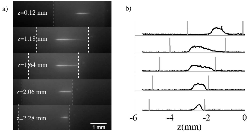
Fig 7. 13: a) Plasma luminescence as the sample approaches the DL and b) corresponding profiles. The iris diameter was 5.5 mm ( NA=0.026 ) and the input energy was 0.76 \mu\text{J} . The vertical gray lines indicate the limits of the crystal.
