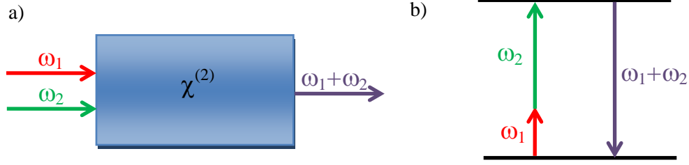
Fig 3. 2: a) Scheme of sum-frequency generation. b) Energy level diagram.
