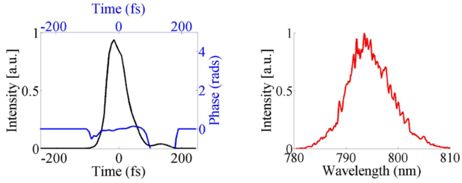
Fig A. 1: a) Pulse in the temporal domain. b) Corresponding spectrum
