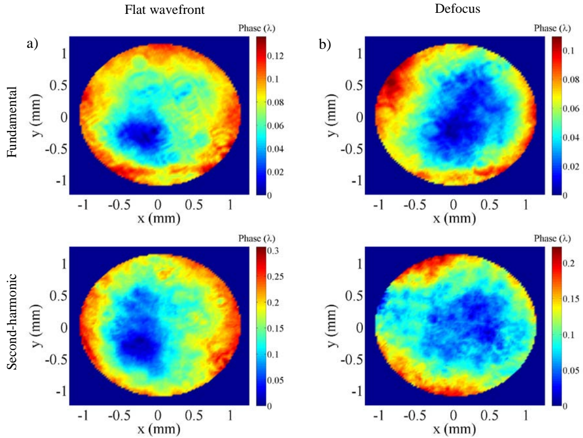
Fig 4. 26: Induced defocus in the SH (bottom) as peak intensity is increased from 0.5 to 34 GW/cm 2 under perfect phase-matching conditions when the incident fundamental pulse (top) presents a) a flat wavefront or b) a focusing wavefront.
