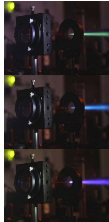
Fig 7. 3: Photography of the SC generated with a DL for different DL-sample distances.
