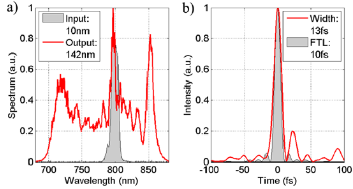
Fig 2. 21: Input and output pulses in a) the spectral domain and b) the temporal domain.
