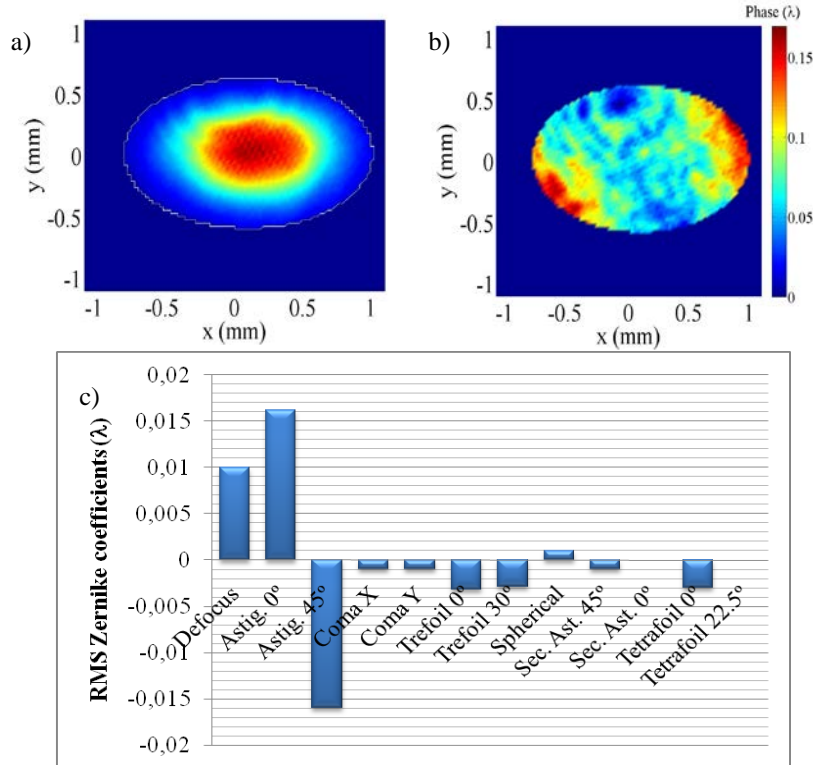
Fig 2. 10: Characterization of the output beam before the stretcher: a) Beam profile, b) wavefront and c) phase decomposition in Zernike polynomials.
