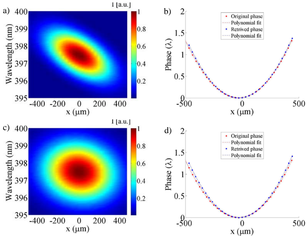
Fig 5. 11: Simulated spectral traces for wavefront measurements with a) 1000 \mu\text{m} and c) 300 \mu\text{m} thick BBO crystal. b), d) Corresponding wavefronts (blue squares) and comparison to the original phase (red squares). The dashed lines represent the fitting with Zernike polynomials.
