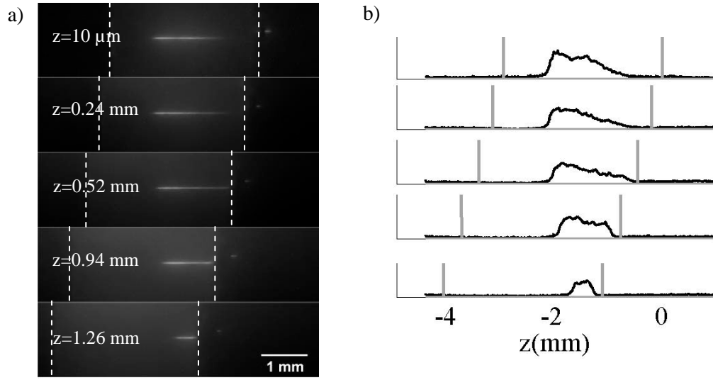
Fig 7. 11: a) Plasma luminescence as the sample approaches the DL and b) corresponding profiles. The iris was fully open and the input energy was 1.20\ \mu\text{J} . The vertical gray lines indicate the limits of the crystal.
