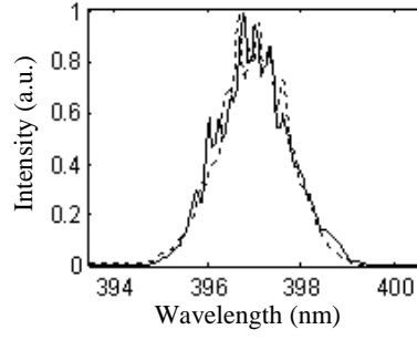
Fig 5. 4: Comparison between the measured SH signal (solid line) and the estimation (dashed line) for the fundamental spectrum applying Eq. (108).
