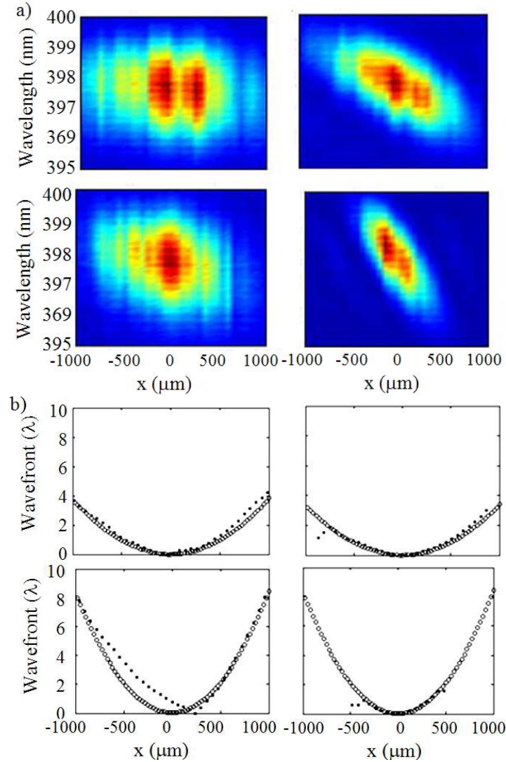
Fig 5. 16: a) Spectral traces for 300 \mu\text{m} (left panel) and 1000 \mu\text{m} (right panel) thick BBO for 0.95\lambda (upper panels) and 1.84\lambda (lower panels) PtV defocus and a 1 mm pupil. All the traces are normalized. b) Experimentally retrieved wavefront (black symbols) and wavefront measured with the commercial sensor (white symbols).
