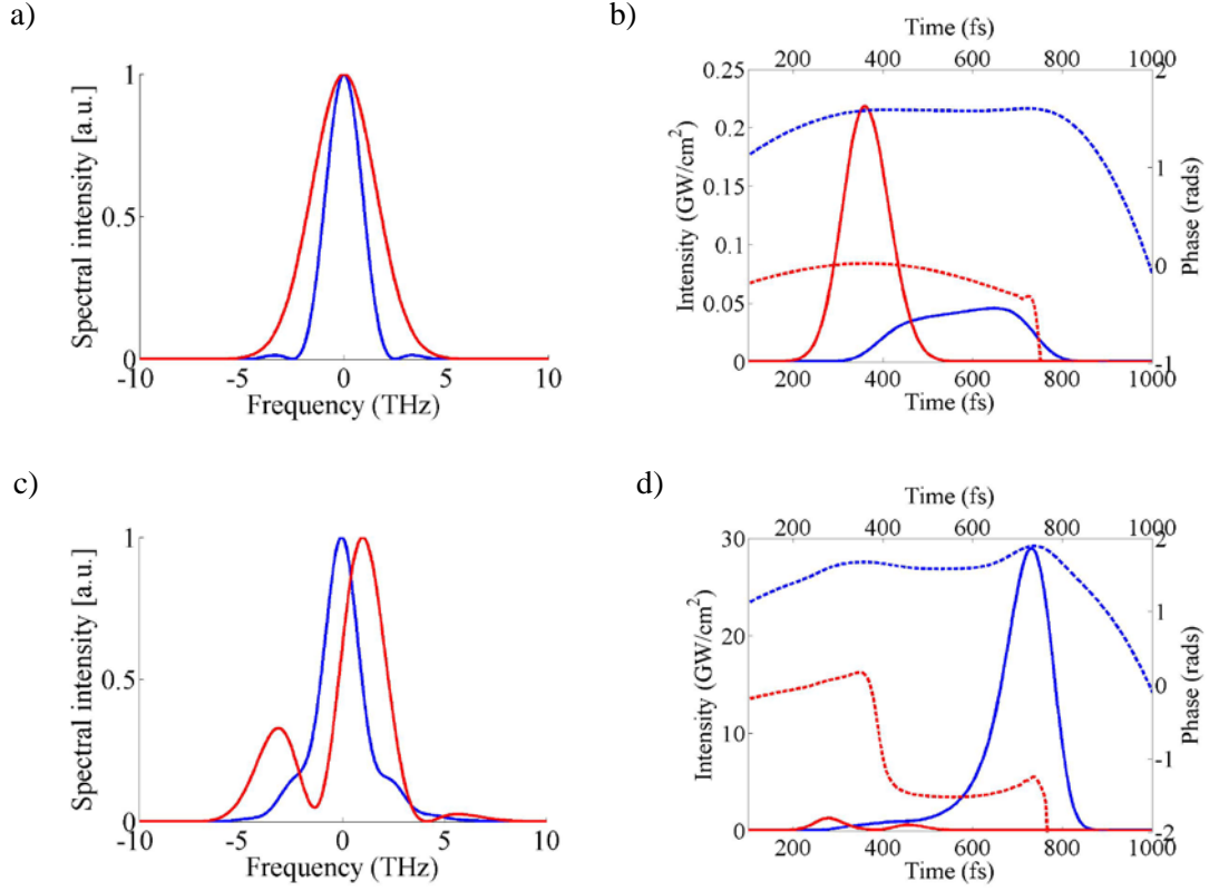
Fig 4. 6: Time and spectral characteristics of the fundamental (red) and the SH (blue). Spectrum for (a) 5 and (c) 320 \mu\text{J} input energy pulses (0.5 and 34 \text{GW}/\text{cm}^2 peak intensity, respectively). Intensity (solid line) and phase (dotted line) for (b) 5 and (d) 320 \mu\text{J} input energy pulses.
