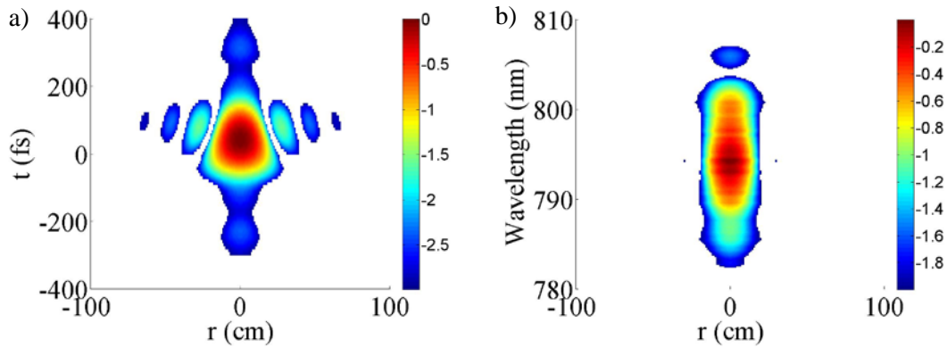
Fig 7. 15: Simulation of the a) spatiotemporal and b) spatio-spectral features at the focus of the DL for the central wavelength when the iris aperture is reduced to 5.5 mm ( \text{NA}=0.026 ). The graphs are plotted in logarithmic scale that comprises three (a) and two (b) orders of magnitude.
