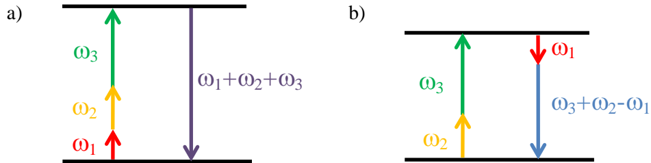
Fig 3. 4: Energy level diagrams for the third-order nonlinear interactions corresponding to a) Eq. (29) and b) Eq. (30)
