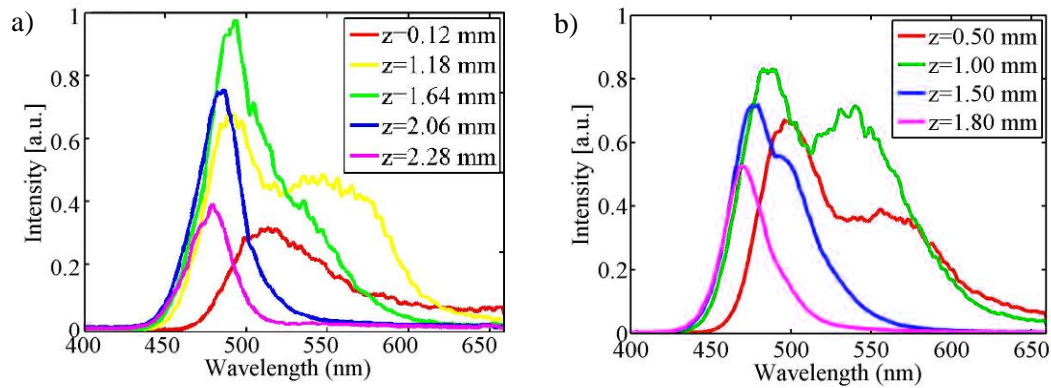
Fig 7. 6: Spectra taken for a) NA=0.026 and pulse energy of 0.98 \mu J and b) NA=0.034 and pulse energy of 1.10 \mu J .
