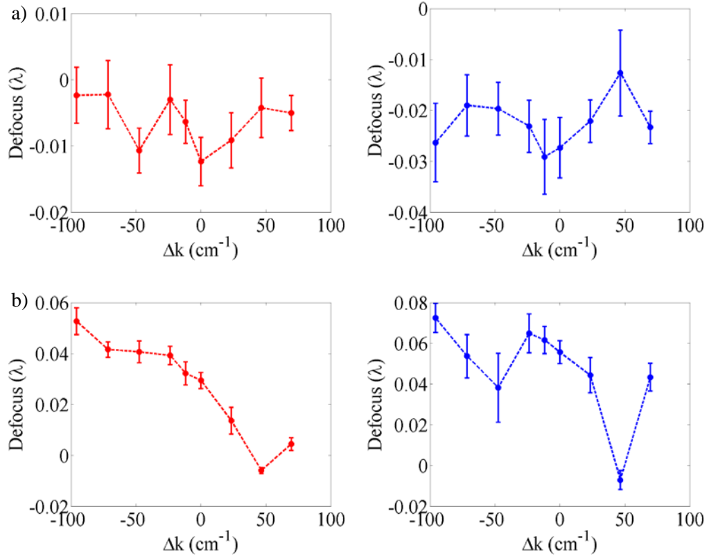
Fig 4. 18: Graphics showing defocus (RMS) as a function of the phase mismatch for the non-converted fundamental (red) and the SH (blue) with a) 5 \mu J and b) 320 \mu J input pulses.
